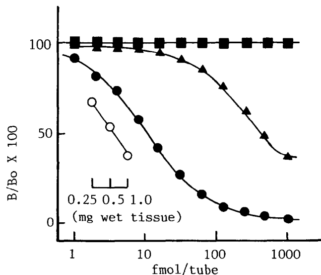
Fig. 1. Standard curve of radioimmunoassay for adrenomedullin and cross-reactivity of antiserum #171CI-9. Inhibition of ^{125}\text{I} -labeled AM(40–52) \text{NH}_2 binding to the antiserum by serial dilutions of AM(1–52) \text{NH}_2 , (45–52) \text{NH}_2 , (47–52) \text{NH}_2 (●), (45–52) \text{COOH} (▲), CGRPs (■), amylin (■) and NPY (■). AM(45–52) \text{COOH} showed 2.5% cross-reactivity with the antiserum. The latter three were derived from human and none exhibited any cross-reactivity with the antiserum. Inhibition of ^{125}\text{I} -labeled AM(40–52) \text{NH}_2 binding to the antiserum by serial dilutions of human adrenal medulla sample (○), is roughly parallel to that of standard AM(1–52) \text{NH}_2 .
